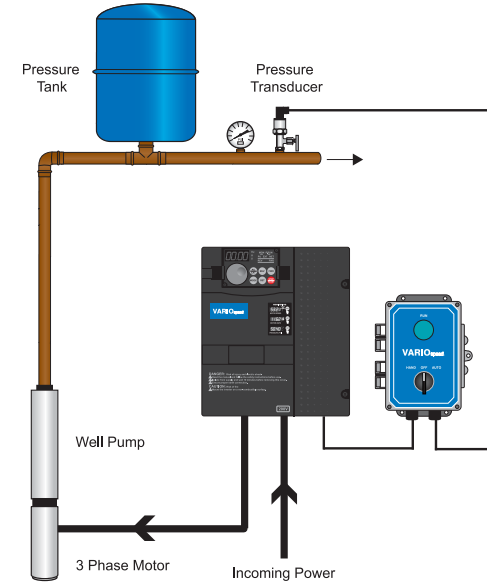
Deep Well Submersible Pump Application
